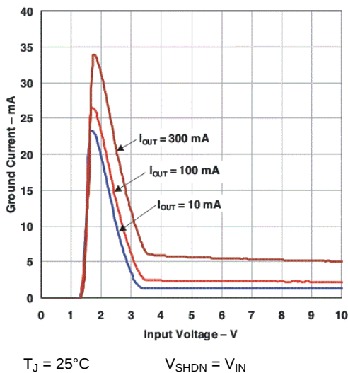
Figure 11. TPS7A4533 Ground Current vs Input Voltage
