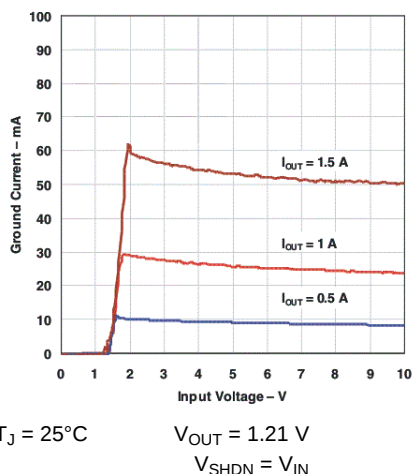
Figure 10. TPS7A4501 Ground Current vs Input Voltage
