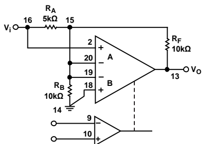
Figure 21. AD630 Symmetric Gain (±2)
