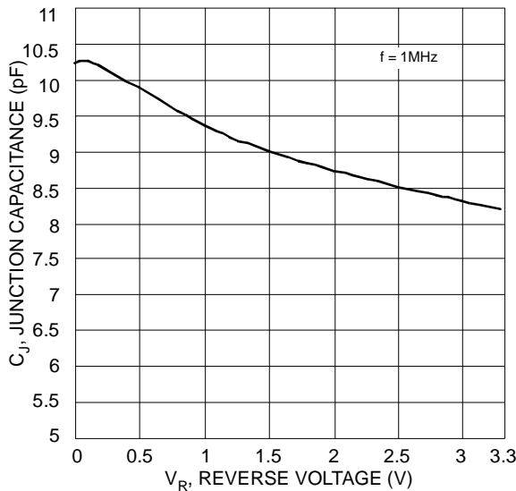
Figure 5 Typical Capacitance
