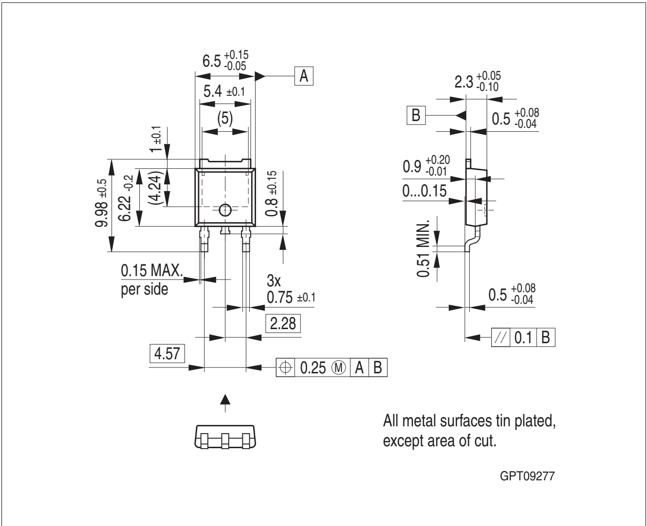
Figure 5 PG-TO252-3
