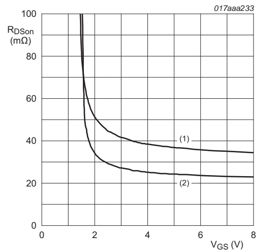
Fig 9. Drain-source on-state resistance as a function of gate-source voltage; typical values I_D = 5\text{ A} (1) T_j = 150\text{ }^\circ\text{C} (2) T_j = 25\text{ }^\circ\text{C}
