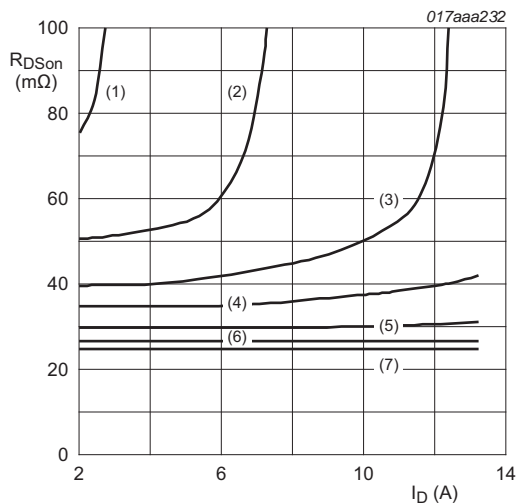
Fig 8. Drain-source on-state resistance as a function of drain current; typical values T_j = 25\text{ }^\circ\text{C} (1) V_{GS} = 1.4\text{ V} (2) V_{GS} = 1.6\text{ V} (3) V_{GS} = 1.8\text{ V} (4) V_{GS} = 2.0\text{ V} (5) V_{GS} = 2.5\text{ V} (6) V_{GS} = 3.0\text{ V} (7) V_{GS} = 4.5\text{ V}
