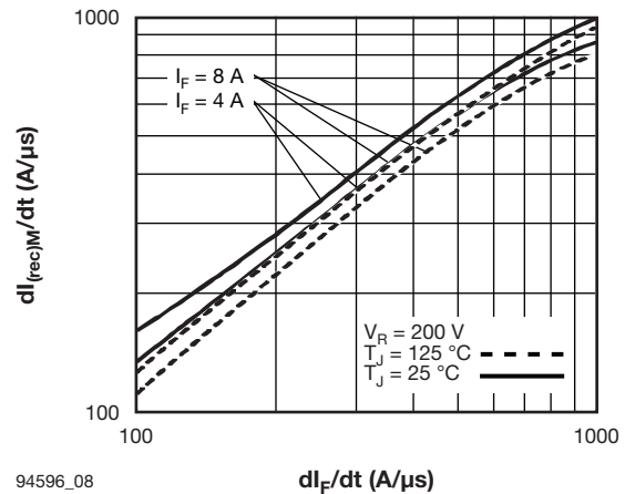
94596_08 Fig. 8 - Typical dI_{(rec)M}/dt vs. di_F/dt
