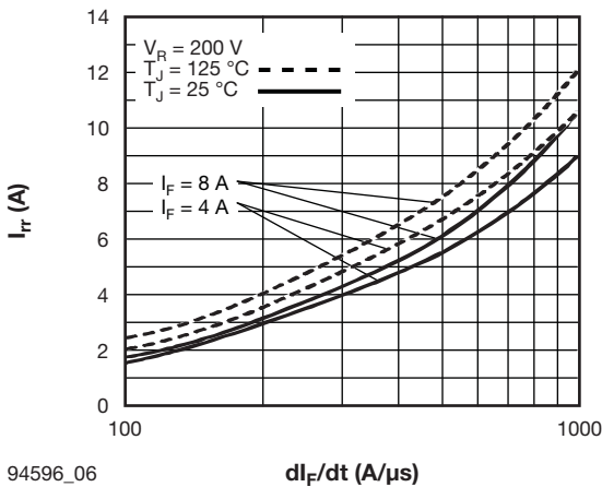
94596_06 Fig. 6 - Typical Recovery Current vs. di_F/dt
