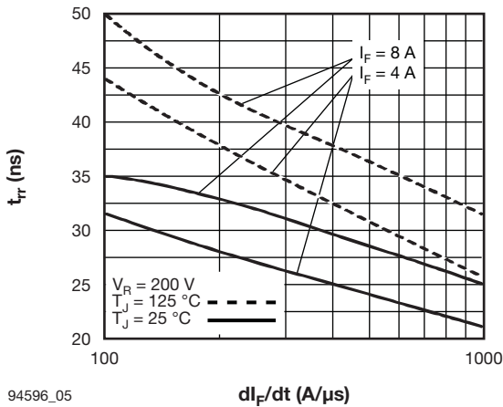
94596_05 Fig. 5 - Typical Reverse Recovery Time vs. di_F/dt
