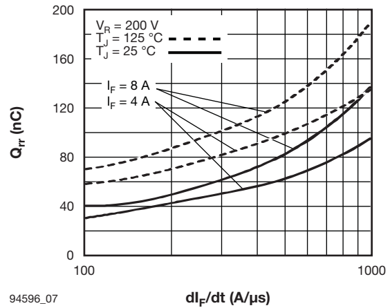
94596_07 Fig. 7 - Typical Stored Charge vs. di_F/dt
