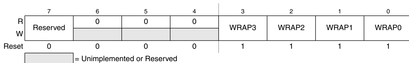
Figure 12-3. ATD Control Register 0 (ATDCTL0)
