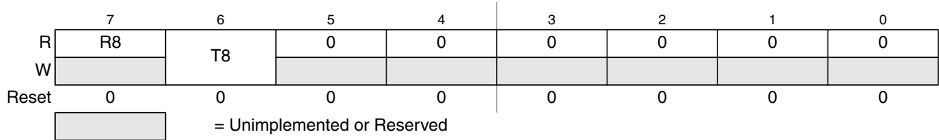
Figure 20-12. SCI Data Registers (SCIDRH)
