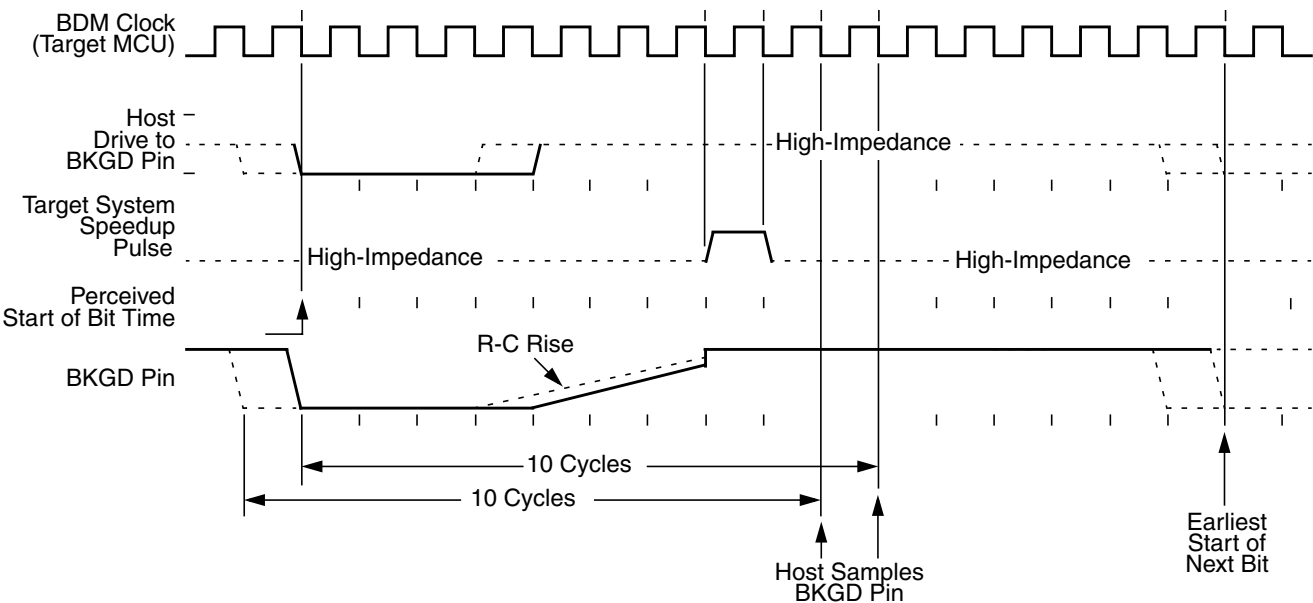
Figure 7-8. BDM Target-to-Host Serial Bit Timing (Logic 1)
