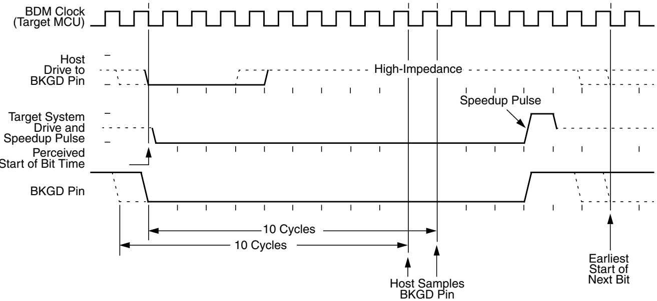
Figure 7-9. BDM Target-to-Host Serial Bit Timing (Logic 0)
