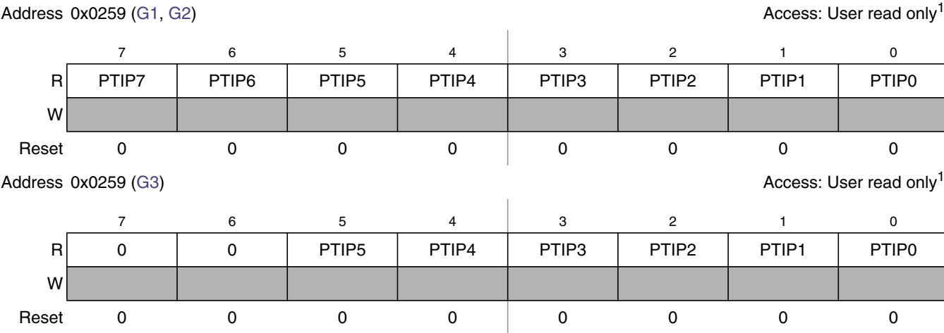
Figure 2-36. Port P Input Register (PTIP)
