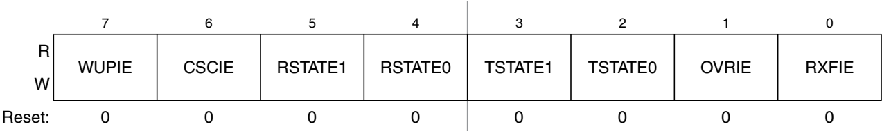
Figure 18-9. MSCAN Receiver Interrupt Enable Register (CANRIER)
