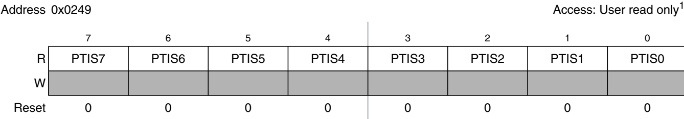
Figure 2-22. Port S Input Register (PTIS)
