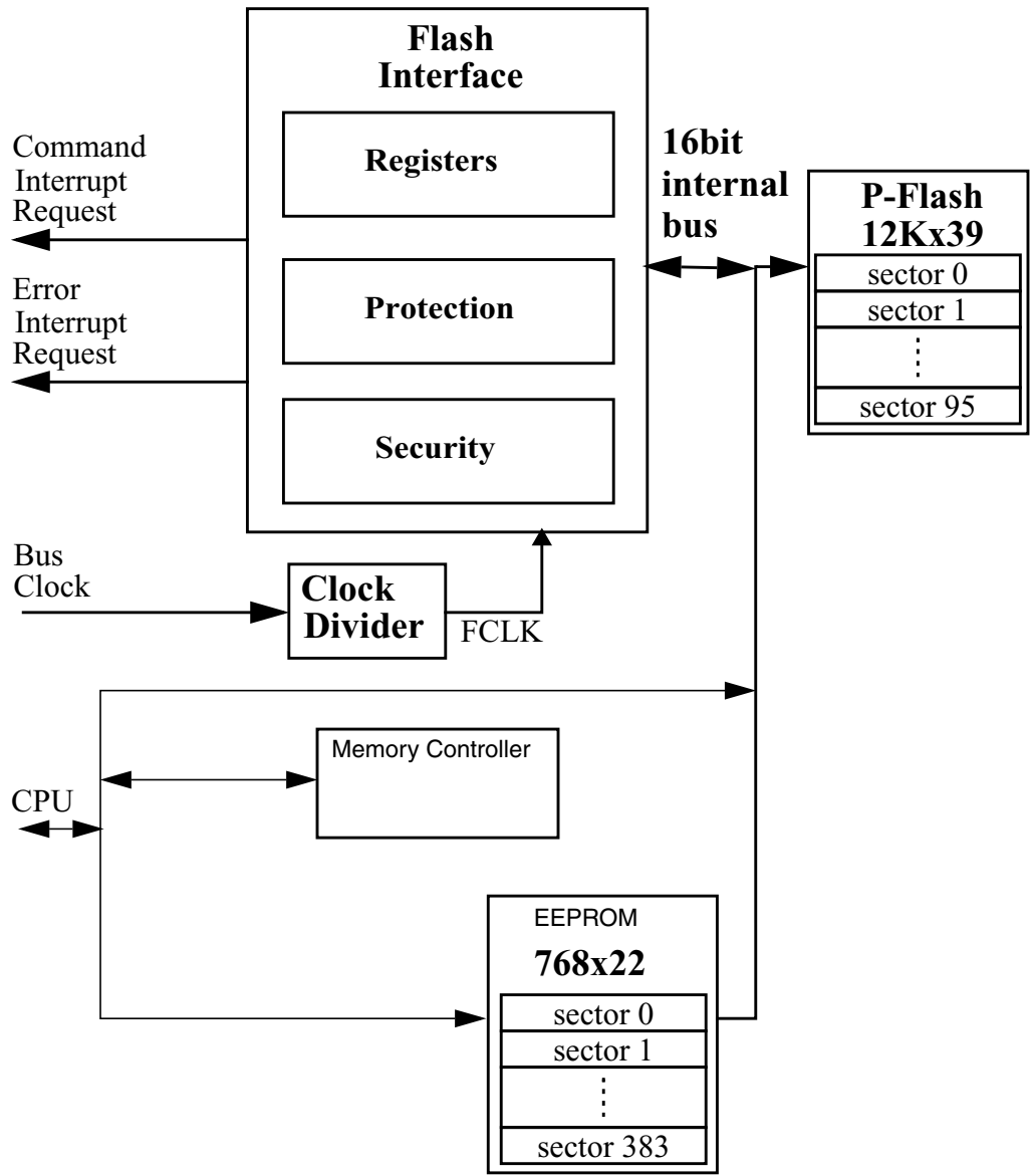
Figure 26-1. FTMRG48K1 Block Diagram
