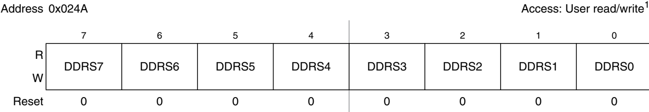
Figure 2-23. Port S Data Direction Register (DDRS)
