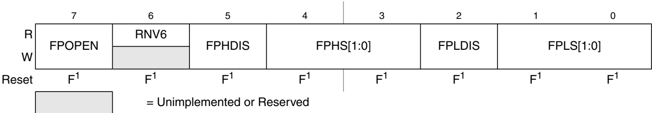
Figure 31-13. Flash Protection Register (FPROT)
