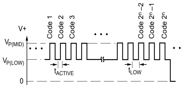
Figure 2. Bit field addressing pulse train. Addressing the bit field by incrementing the code causes the programmable parameter value to change. The number of bits available for a given programming code, n , varies among parameters; for example, the bit field for Sensitivity has 8 bits available, which allows 255 separate codes to be used.
