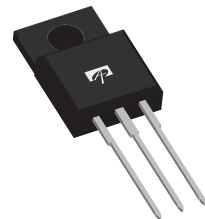
TO-220F (10.16x15.87) (28.86 w/leads)
