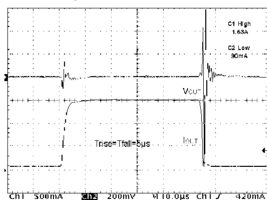
Figure 27. Load transient
