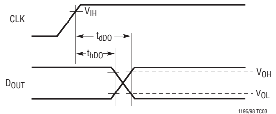
Voltage Waveform for D_{OUT} Delay Time, t_{dDO} , t_{hDO}
