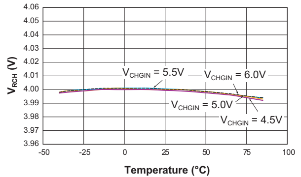
Recharge Voltage Threshold vs. Temperature ( V_{RCH} set to 4.0V by I^2C )
