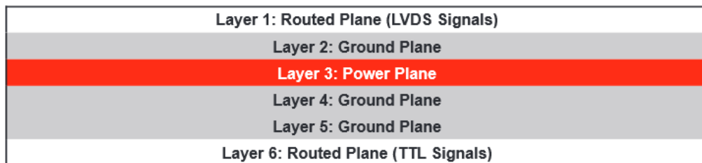
Figure 27. Six-Layer PCB Board
