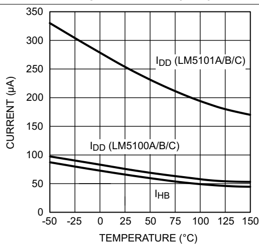
Figure 11. Quiescent Current vs Temperature
