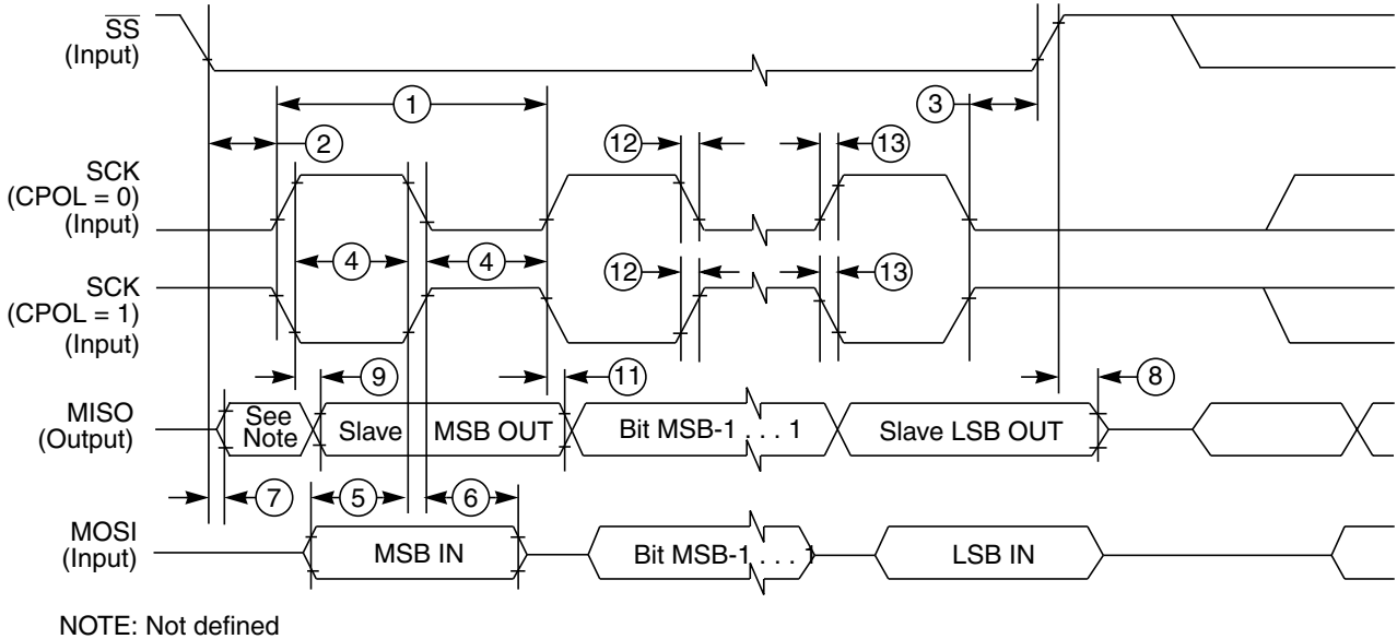
Figure A-10. SPI Slave Timing (CPHA = 1)
