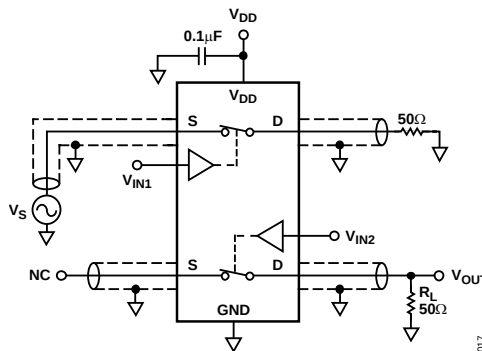
Figure 16. Channel-to-Channel Crosstalk
