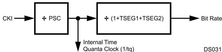
Figure 19-14. CAN Prescaler
