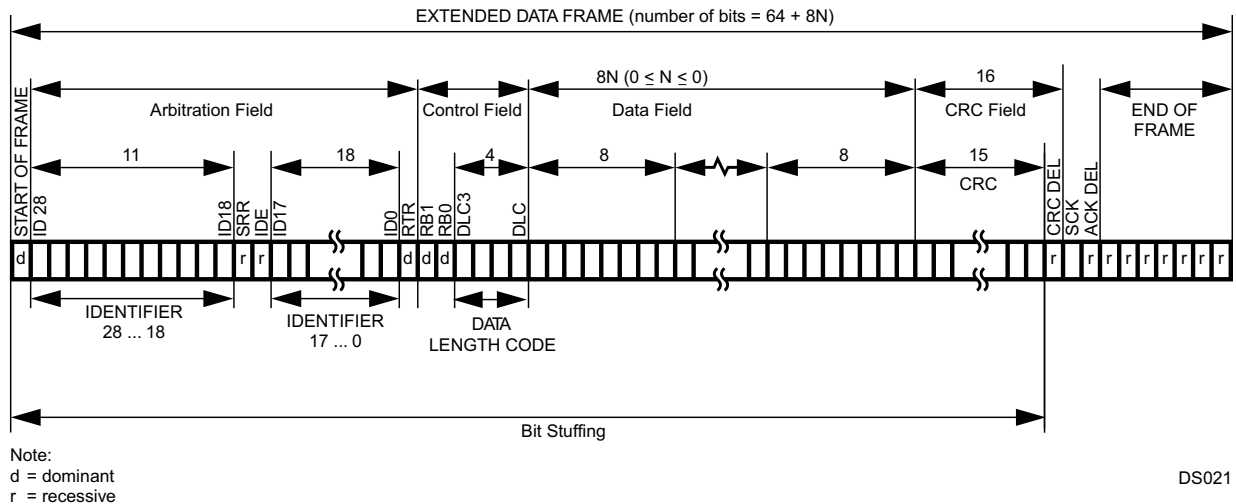
Figure 19-4. Extended Data Frame
