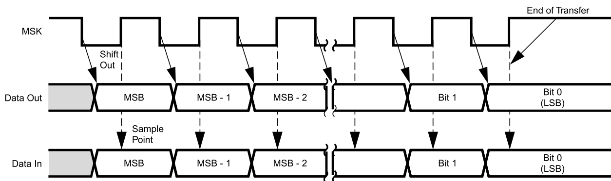
Figure 23-3. Normal Mode (SCIDL = 0)
