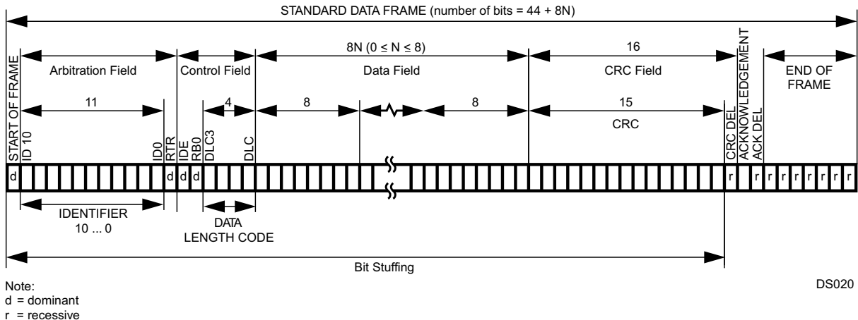
Figure 19-3. Standard Data Frame
