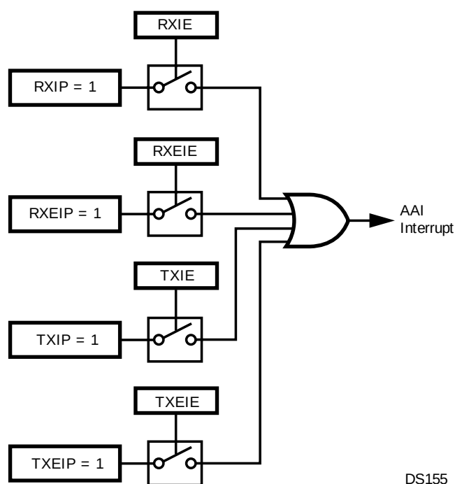
Figure 20-6. AAI Interrupt Structure
