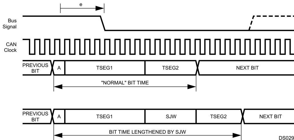
Figure 19-12. Resynchronization ( e > SJW )
