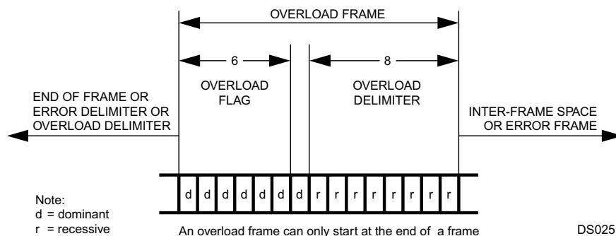
Figure 19-8. Overload Frame
