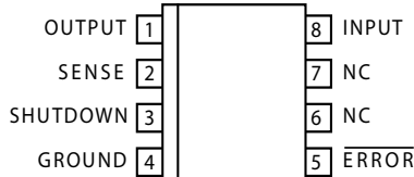
MIC29201-3.3BM (SOIC-8)
