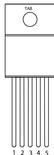
MIC29201/29202BT (TO-220-5)
