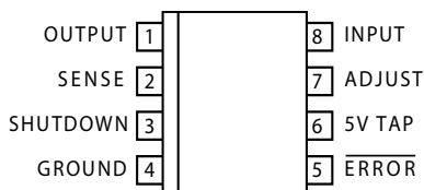
MIC29201-3.3BM (SOIC-8)
