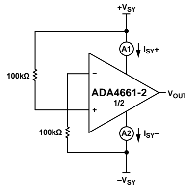
Figure 76. Comparator B
