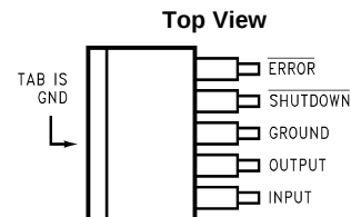
Figure 2. Plastic Surface Mount Package 5-Lead DPAK/TO-263 Package See Package Number KTT0005B
