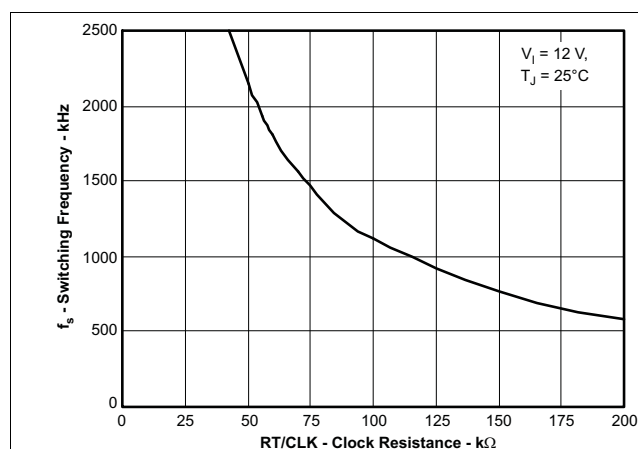
Figure 39. Switching Frequency vs RT/CLK Resistance High Frequency Range
