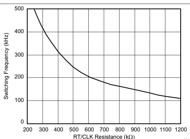
Figure 40. Switching Frequency vs RT/CLK Resistance Low Frequency Range
