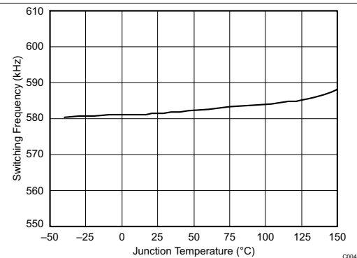
Figure 4. Switching Frequency vs Junction Temperature
