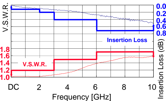
Normally closed (Unmated condition)
