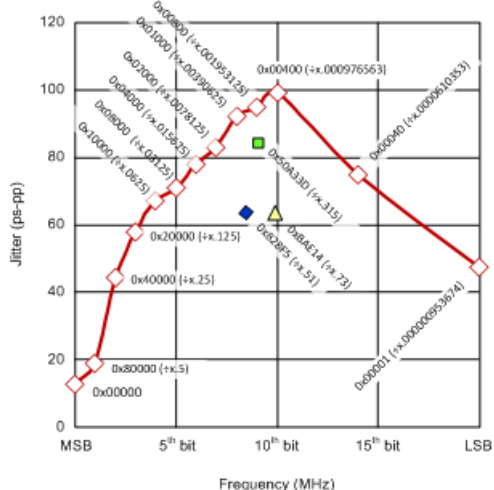
Figure 4. Fractional Divider Bit Selection Impact on Jitter ( f_{ERAC} = 300 MHz)
