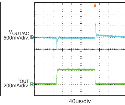
Load Transient with Resistive Load I_{OUT}=10mA-250mA
