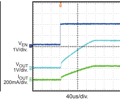
EN Start Up with Resistive Load I_{OUT}=250mA
