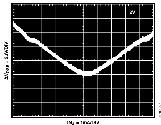
Figure 27. Crosstalk Under Forced Source and Sink Conditions
