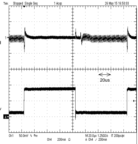
Figure 64. Load transient response 50mA to 350mA tr=tf=100ns , MODE : Low
