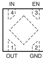
DQN Package 4-Pin X2SON Top View
