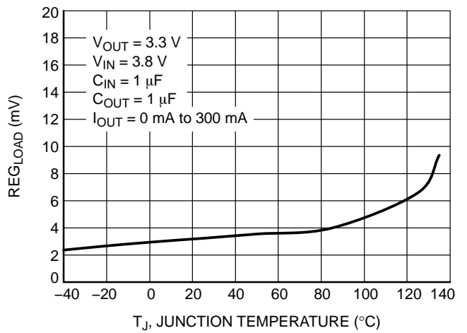
Figure 22. Load Regulation vs. Temperature – 3.3 V
