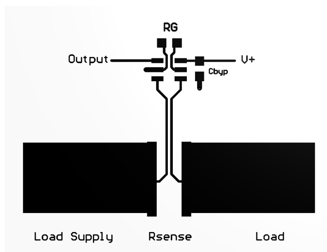
Figure 25. Layout Example
