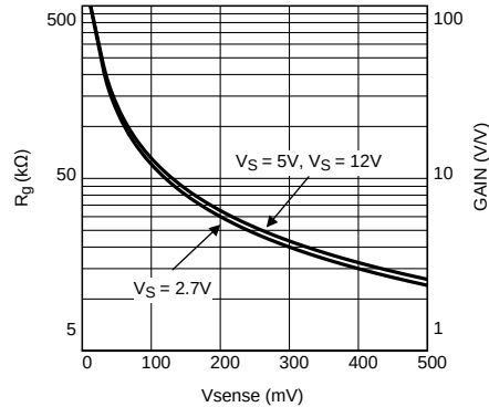
Figure 17. Allowed Gains for Range 1
