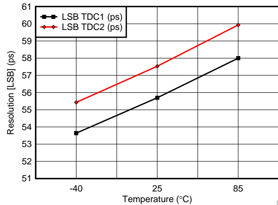
Figure 9. Resolution (LSB) vs Temperature
