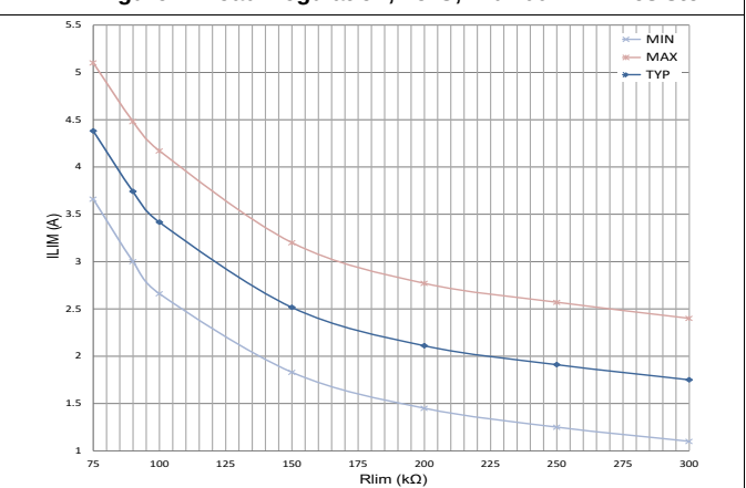
Figure 6. Current Limit V_{IN} = 12\text{ V} , f_{SW} = 500\text{ KHz}
