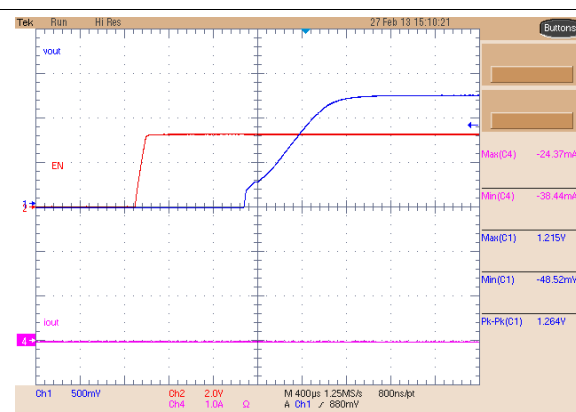
Figure 26. Buck 1 Soft-Start
