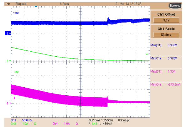
Figure 70. Buck 3 PFM to PWM Transition
