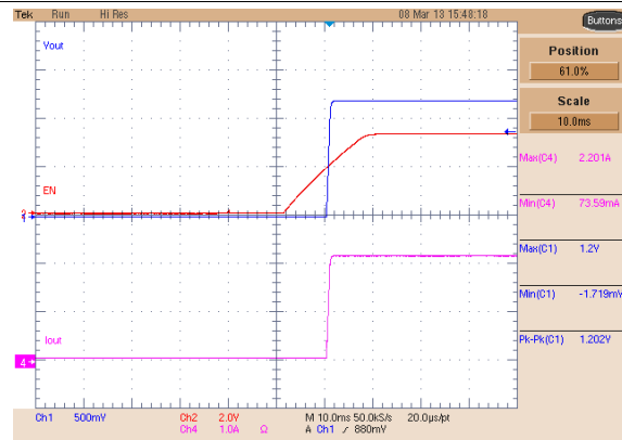
Figure 28. Buck 1 Soft-Start 2-A Load
