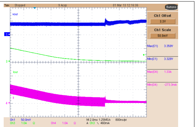
Ch1 = V_{OUT} Ch3 = I_{OUT} Ch4 = Inductor
