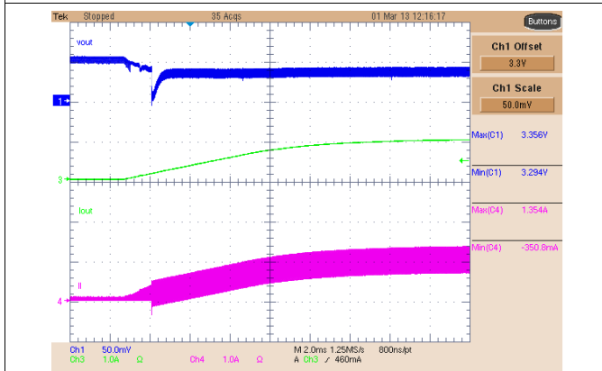
Ch1 = V_{OUT} Ch3 = I_{OUT} Ch4 = Inductor
