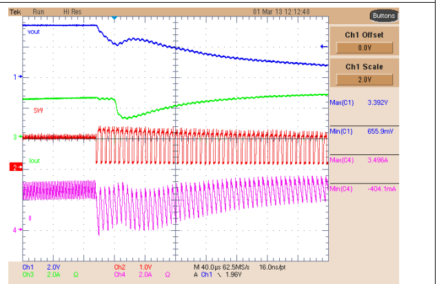
Ch1 = V_{OUT} Ch2 = COMP1 Ch3 = I_{OUT} Ch4 = Inductor
