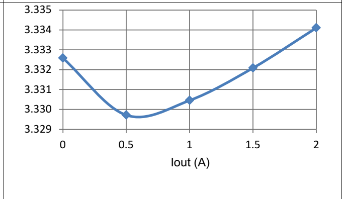
Figure 16. Load Regulation, 25°C, 1% 100-PPM Resistor
