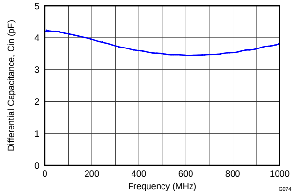
Figure 113. ADC Analog Input Capacitance (C IN ) Across Frequency
