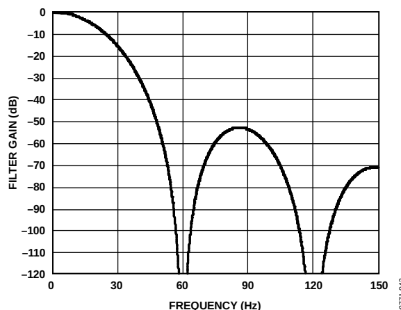
Figure 29. \text{Sinc}^4 Filter Response (FS[9:0] = 80)
