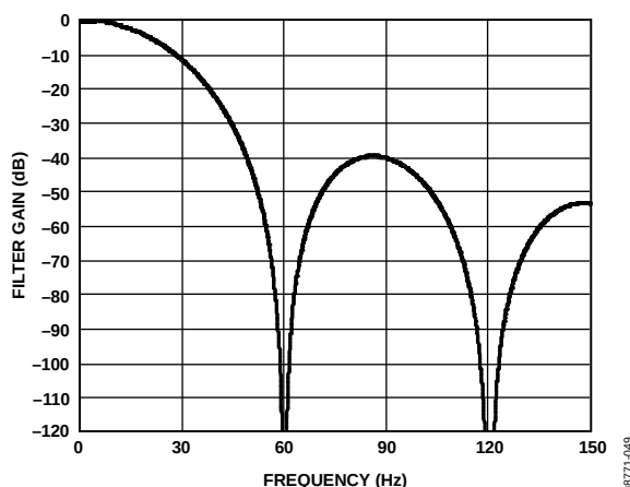
Figure 37. Sinc 3 Filter Response (FS[9:0] = 80)
