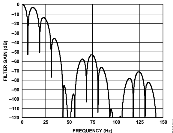
Figure 43. Sinc 4 Filter Response (FS[9:0] = 96, Chop Enabled)
