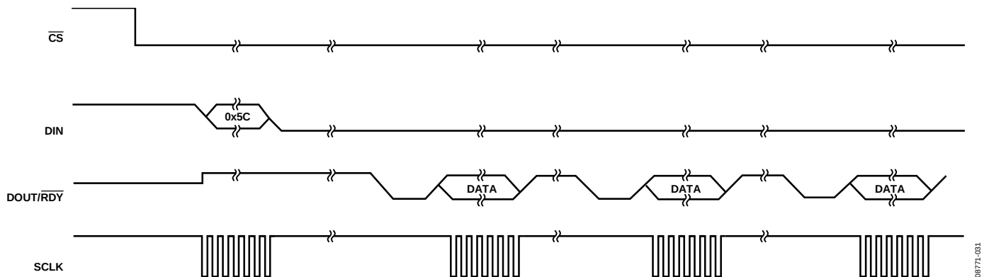
Figure 23. Continuous Read
