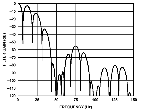
Figure 44. Sinc 4 Filter Response (FS[9:0] = 96, Chop Enabled, REJ60 = 1)
