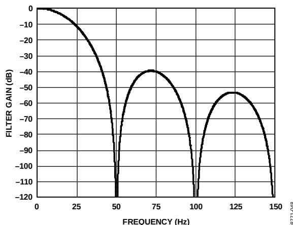
Figure 36. Sinc 3 Filter Response (FS[9:0] = 96)
