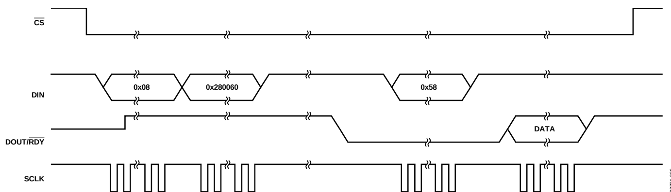
Figure 21. Single Conversion
