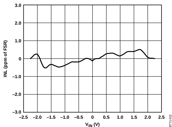
Figure 12. INL (Gain = 1)
