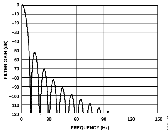
Figure 30. \text{Sinc}^4 Filter Response (FS[9:0] = 480)
