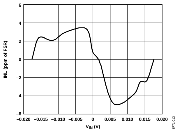
Figure 13. INL (Gain = 128)
