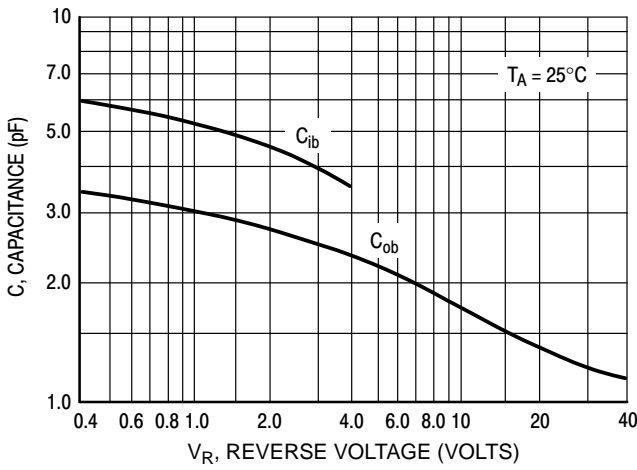
Figure 8. Capacitances
