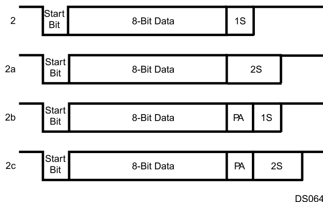
Figure 21-5. 8-Bit Data Frame Options
