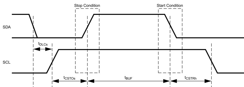
Figure 29-16. ACB Signals (SDA and SCL) Timing
