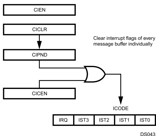
Figure 18-26. Interrupt Management
