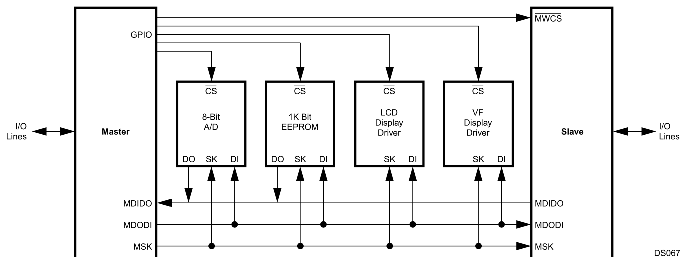
Figure 22-1. Microwire Interface
