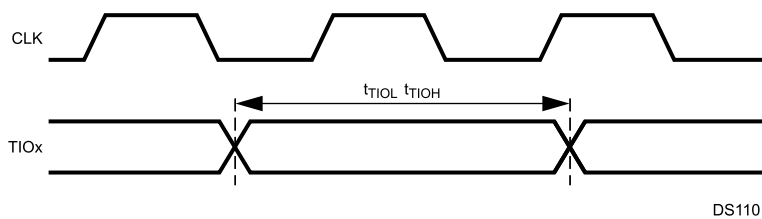
Figure 29-21. Versatile Timing Unit Input Timing
