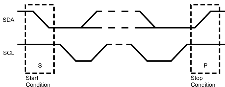
Figure 23-2. Start and Stop Conditions
