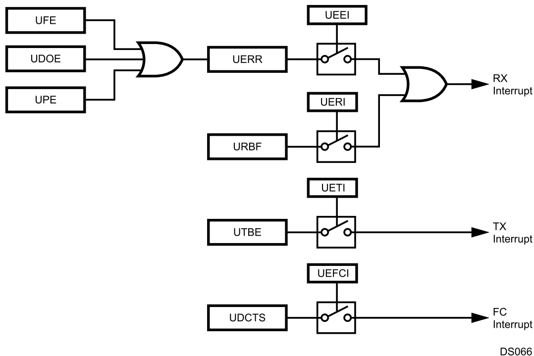
Figure 21-7. UART Interrupts
