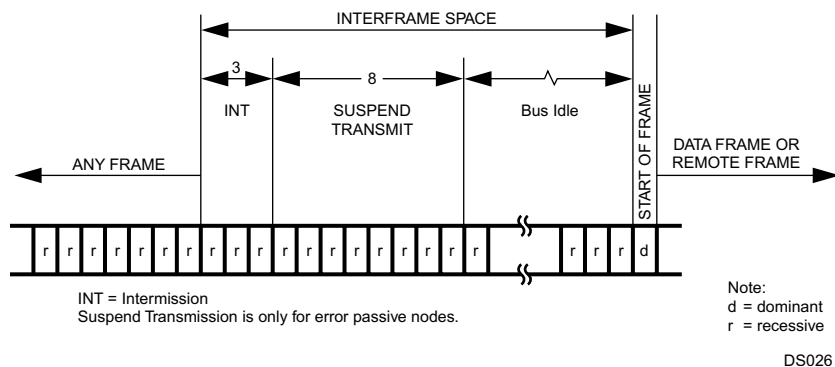
Figure 18-9. Interframe Space
