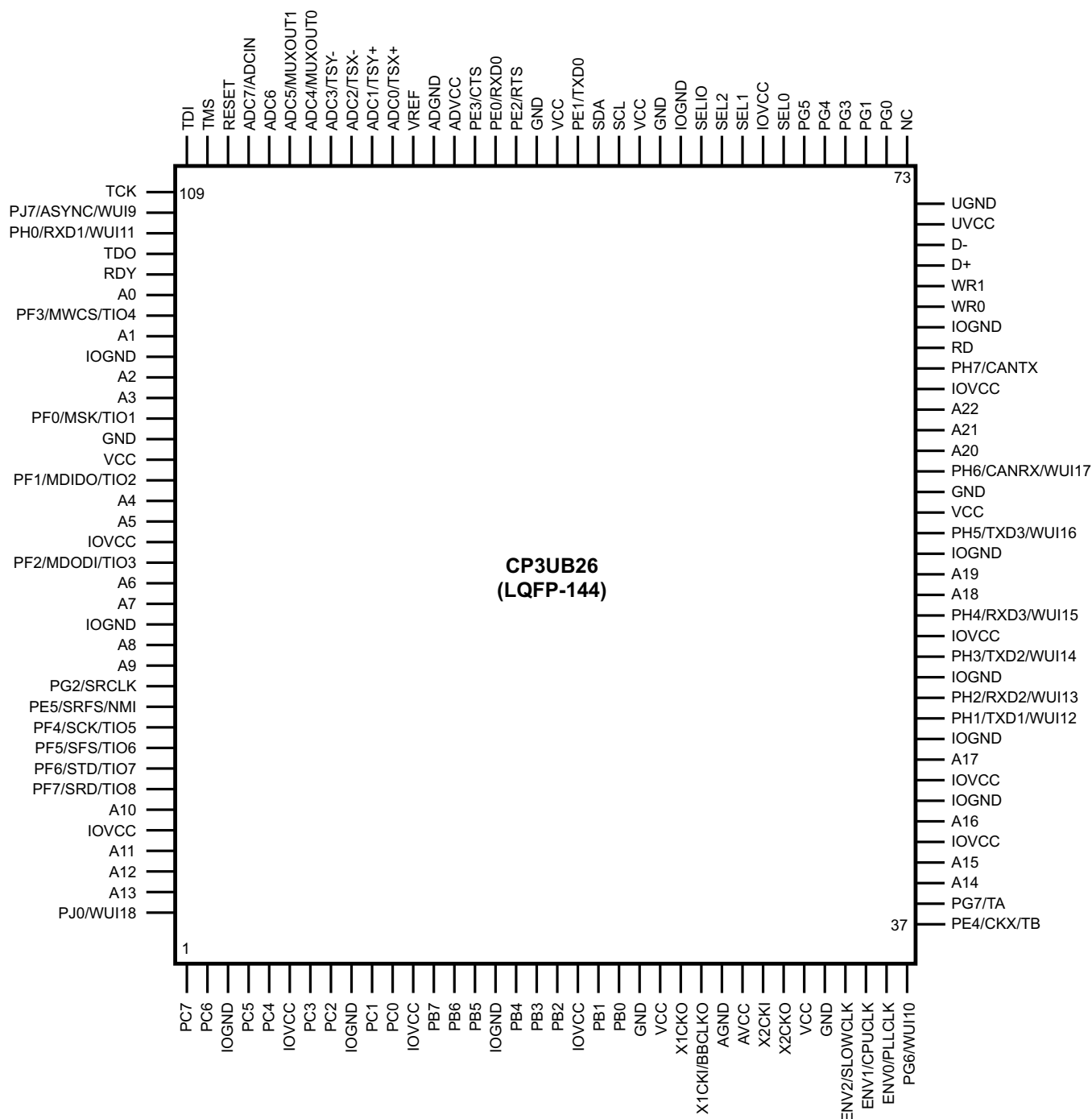
Figure 30-2. CP3UB26 in the LQFP-144 Package (Top View)
