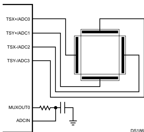
Figure 15-2. Touchscreen Interface
