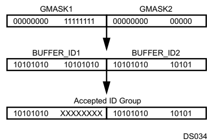
Figure 18-17. Acceptance of a Group of Identifiers
