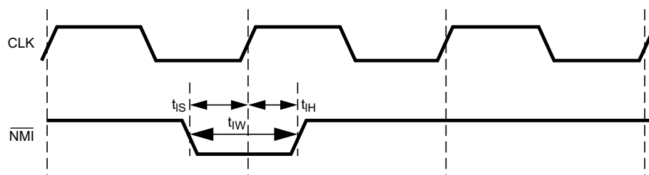
Figure 29-2. \overline{\text{NMI}} Signal Timing
