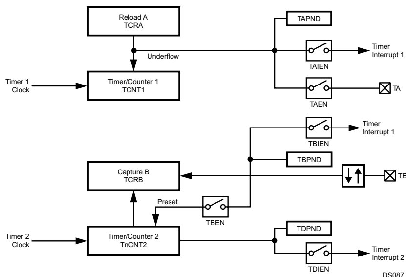
Figure 25-7. Input Capture Plus Timer Mode
