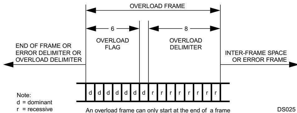
Figure 18-8. Overload Frame
