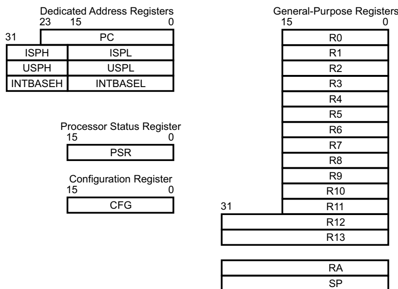
Figure 5-1. CPU Registers
