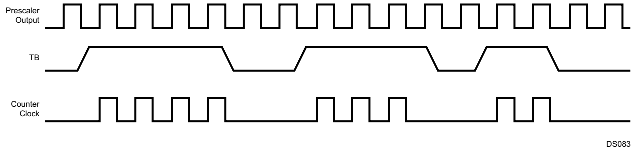
Figure 25-3. Pulse-Accumulate Mode
