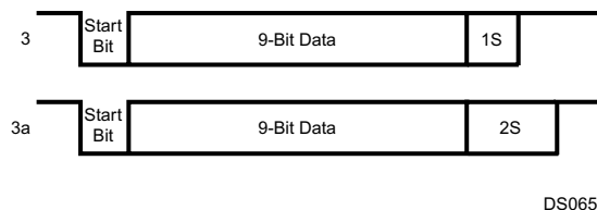
Figure 21-6. 9-bit Data Frame Options
