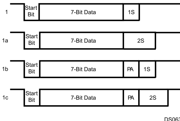
Figure 21-4. 7-Bit Data Frame Options
