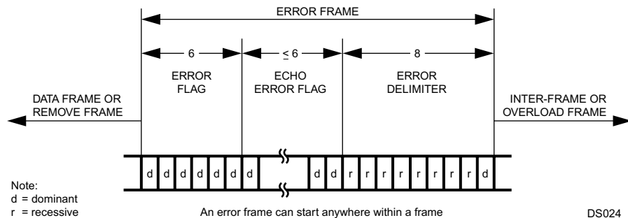
Figure 18-7. Error Frame
