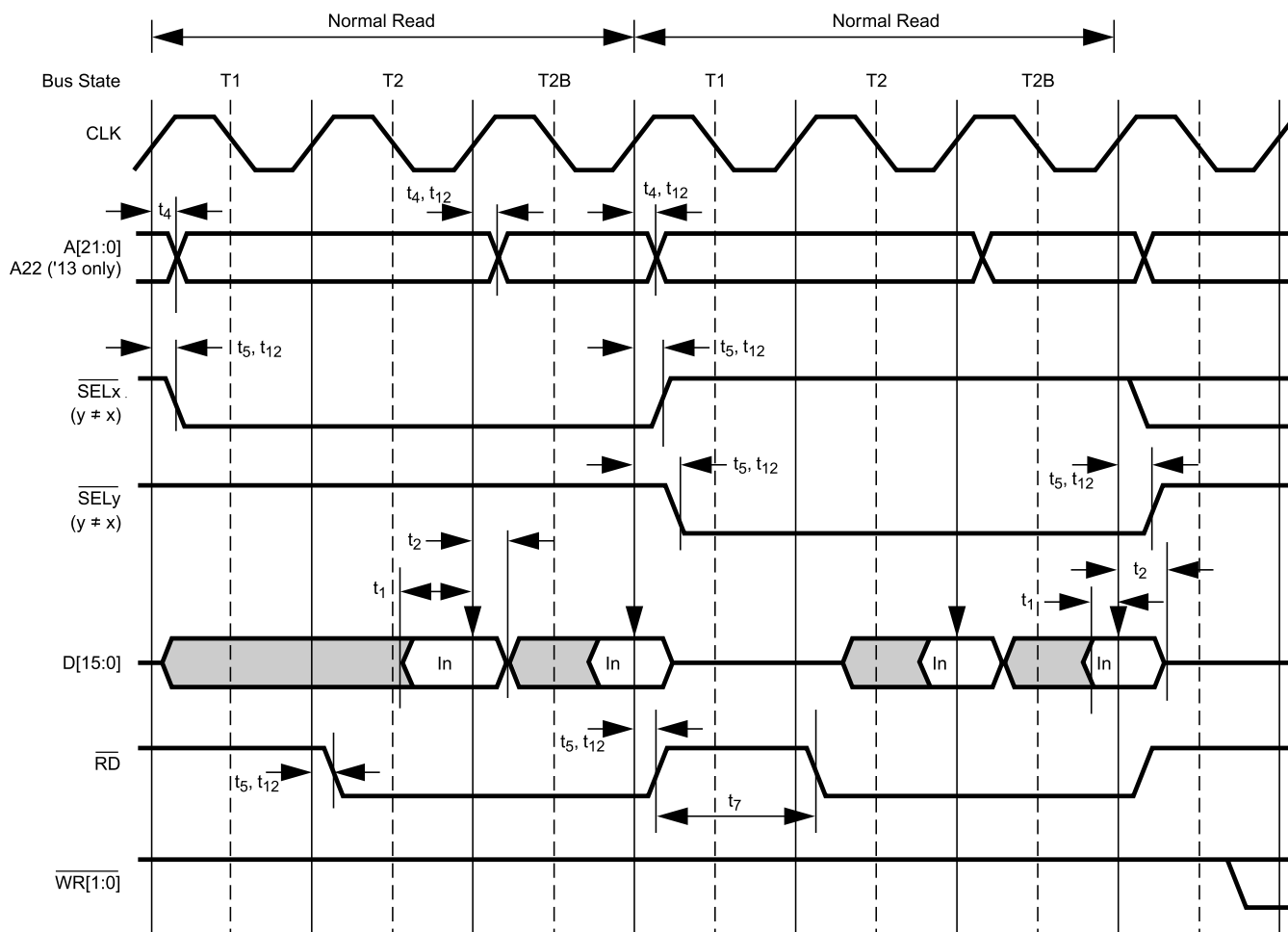
Figure 29-24. Consecutive Normal Read Cycles (Burst, No Wait States)
