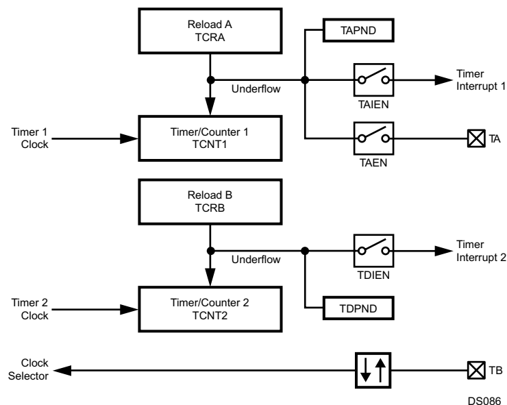
Figure 25-6. Dual-Independent Timer/Counter Mode
