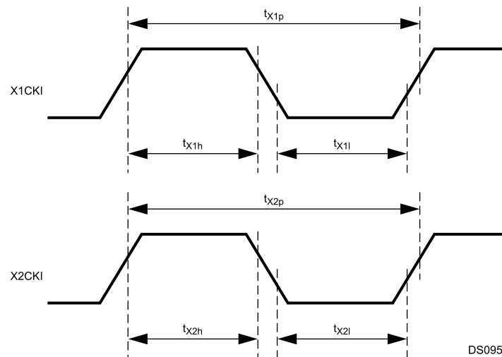
Figure 29-1. Clock Timing
