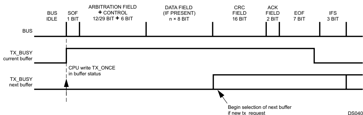
Figure 18-23. Data Transmission
