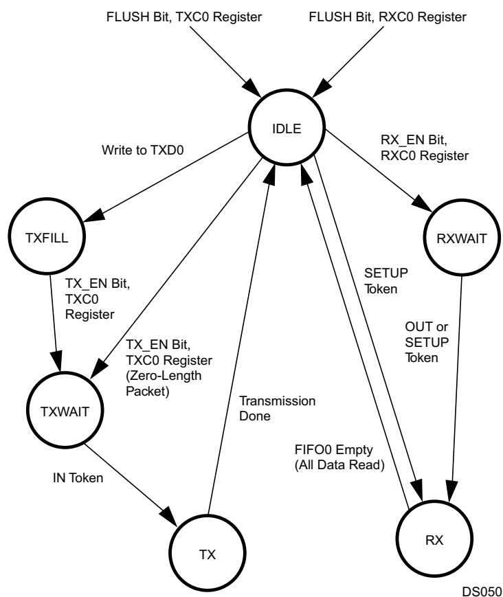
Figure 17-2. Endpoint 0 Operation
