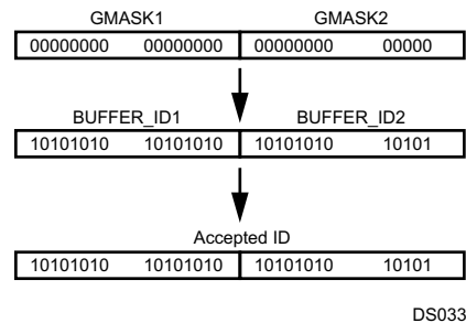
Figure 18-16. Acceptance of a Single Identifier
