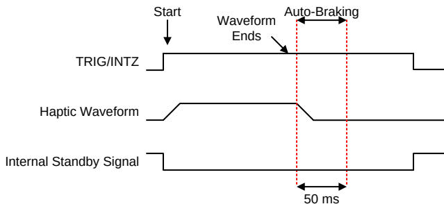
Figure 32. Waveform Sequencer with Trigger-Level Behavior when TRIG/INTZ Pin Left High
