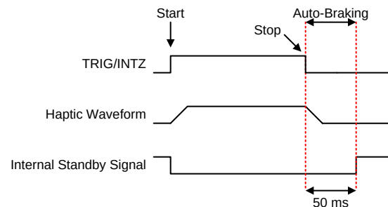
Figure 35. Playback Start and stop Trigger (Level)(RTP or Waveform Sequencer)
