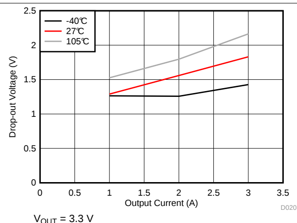
Figure 38. Drop-out for \geq 1.85\text{ MHz}
