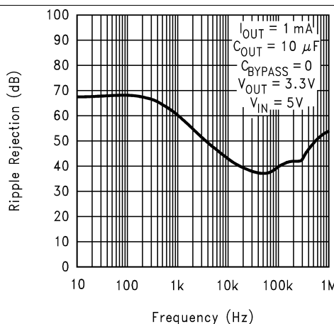
Figure 6. Ripple Rejection
