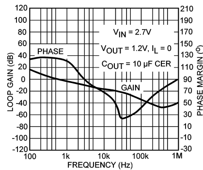
Figure 15. Gain-Bandwidth Plot for No Load
