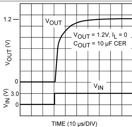
Figure 20. Turnon Time
