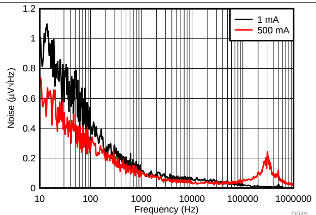
Figure 46. LP5912-0.9 Noise vs Frequency
