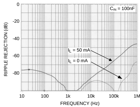
Figure 7. Power Supply Rejection Ratio V_{IN}
