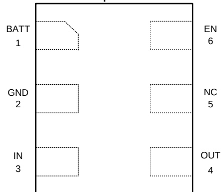
NKH Package 6-Pin USON Top View
