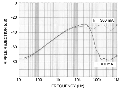
Figure 8. Power Supply Rejection Ratio V_{BATT}
