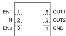
TLV710 TLV711 1.5mm × 1.5mm SON-6 (TOP VIEW)
