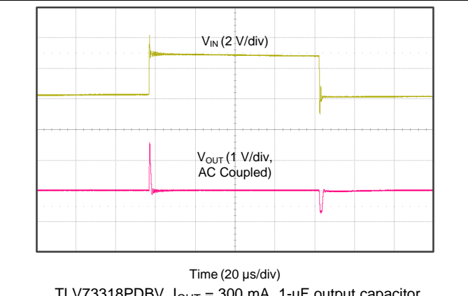
Figure 24. Line Transient
