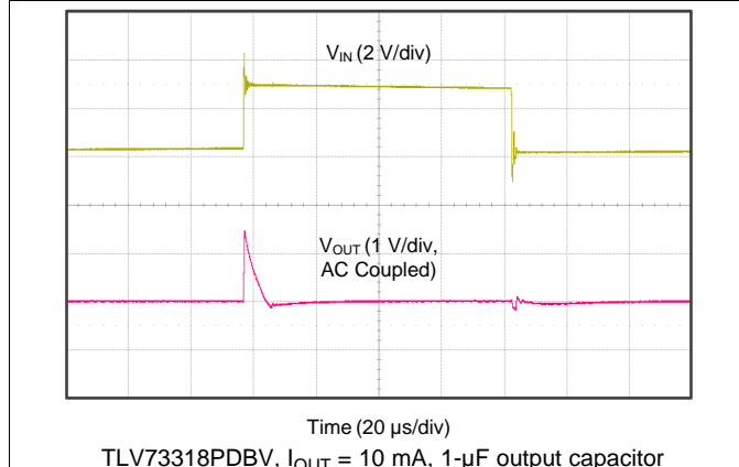
Figure 23. Line Transient
