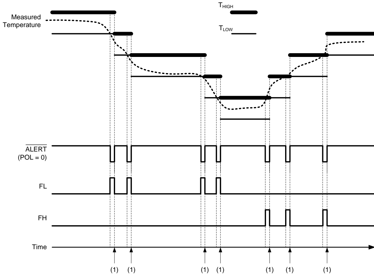
Figure 10. Interrupt Mode
