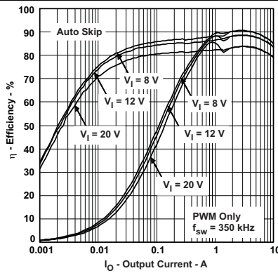
Figure 13. 1.05-V Efficiency vs Output Current
