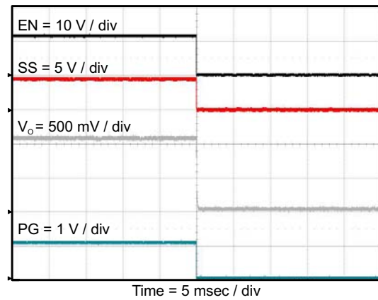
Figure 29. TPS562219 Shut Down Relative To EN
