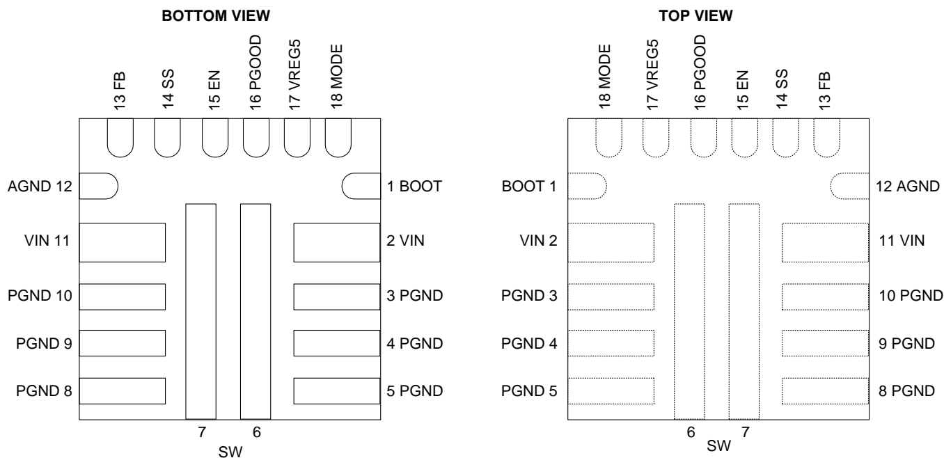
Pin Functions
