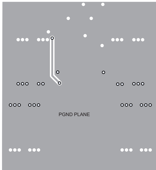
Figure 44. Bottom Layer Layout
