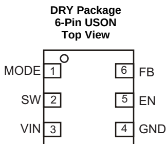
Pin Functions
