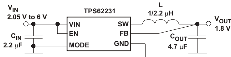
Figure 53. TPS62231 1.8-V Output
