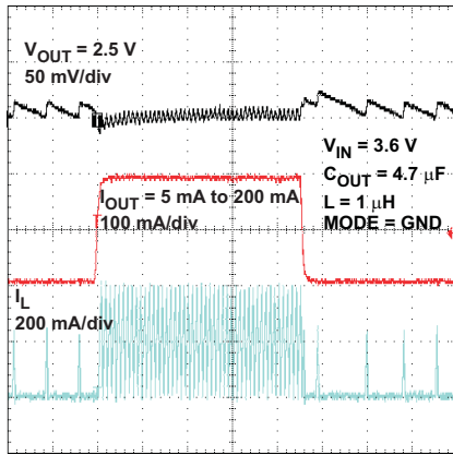
Figure 51. Load Transient Response 5 mA to 200 mA, PFM to PWM Mode, V_{OUT} 2.5 V – TPS62230
