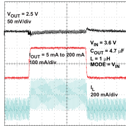
Figure 52. Load Transient Response 5 mA to 200 mA, Forced PWM Mode, V_{OUT} 2.5 V – TPS62230
